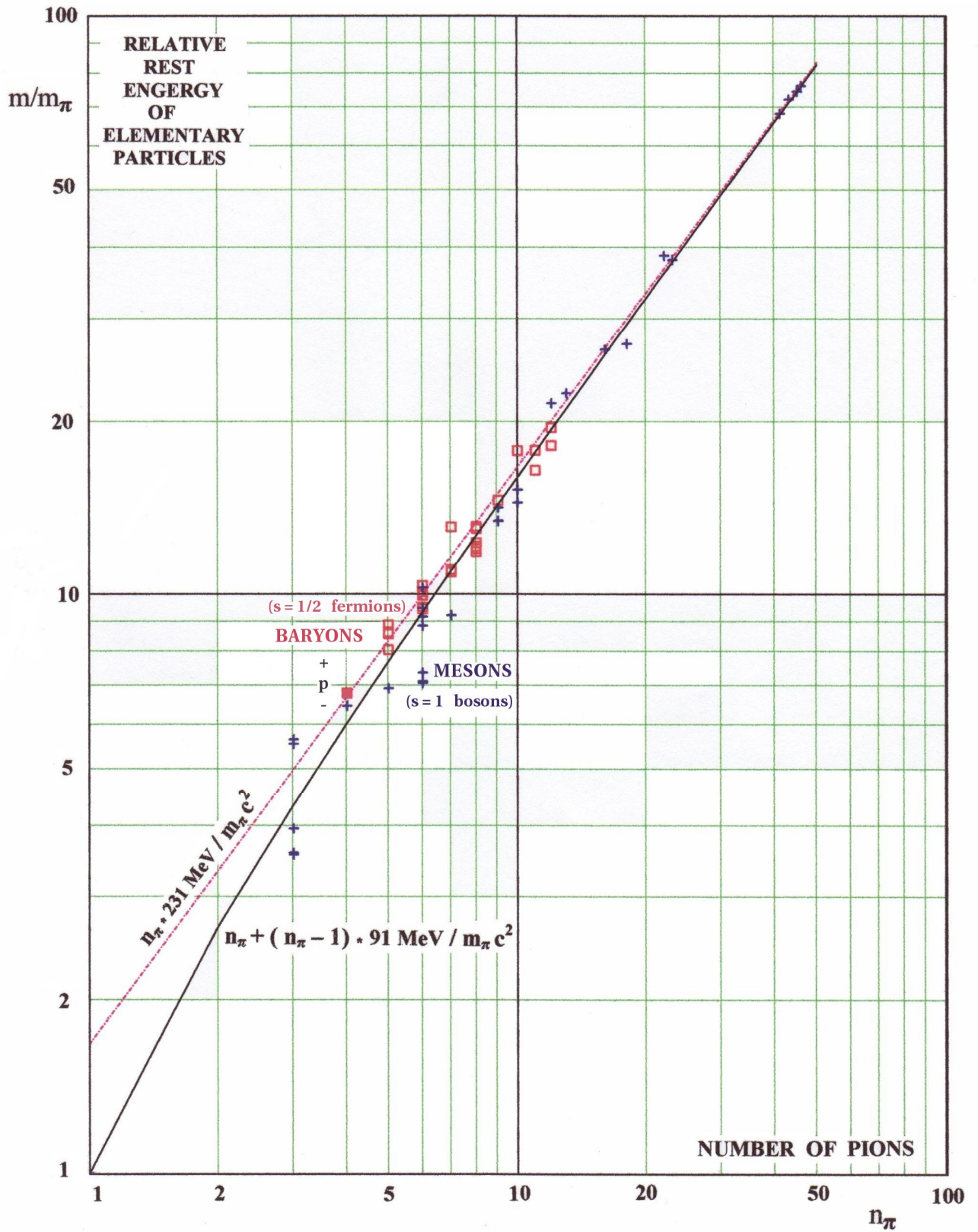
FIG 4: ELEMENTARY PARTICLES AS MULTIPLE PION STATES MASS CORRELATION OF HADRONS WITH PION NUMBER
