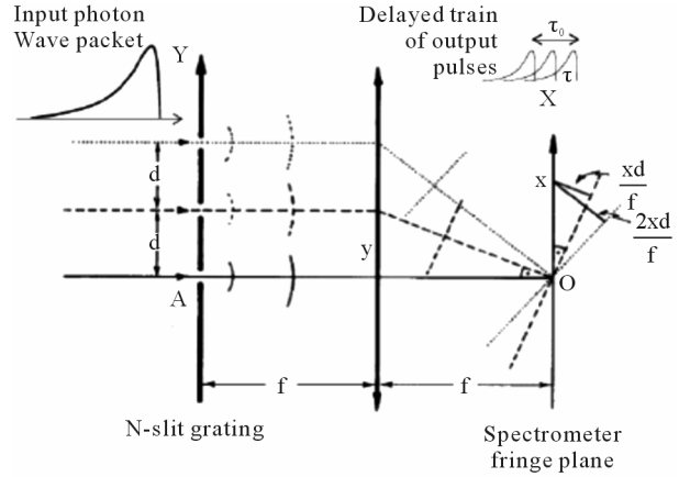
Figure 1. Pulse replication by grating and their temporally delayed superposition by a lens L in on a detector at the measurement plane.
