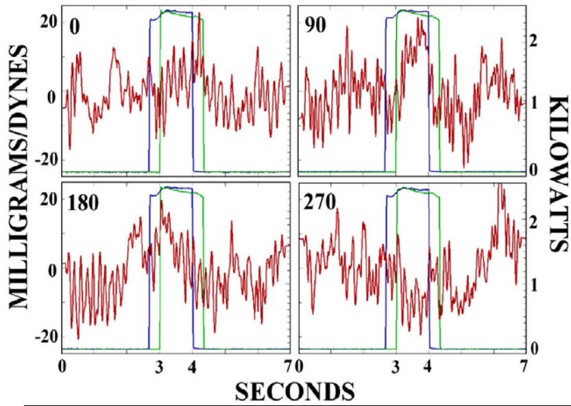
Figure 7: Results for the four relative phase angles of the inductor current and capacitor voltage.
