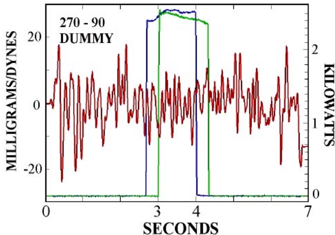
Figure 13: The currents emulation results for the dummy circuit in Figure 12.
