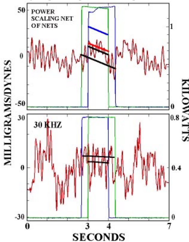
Figure 14: The results for the power scaling test (upper panel) and frequency/power scaling test (lower panel).
