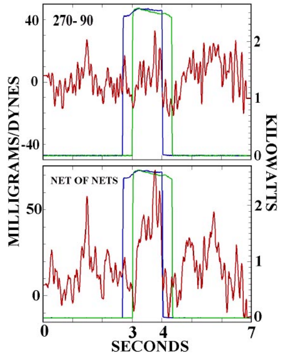
Figure 10: 270 minus 90 degrees results for reversed inductor polarity and those results with the other polarity subtracted.
