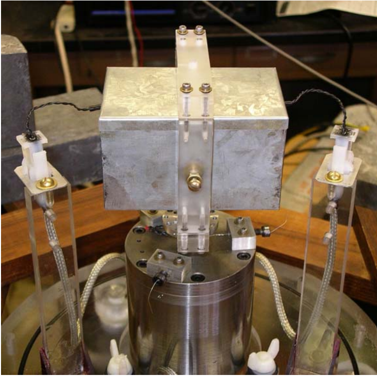
Figure 5: The Faraday cage (steel box) mounted atop the thrust/weight sensor (in the cylindrical steel shield).
