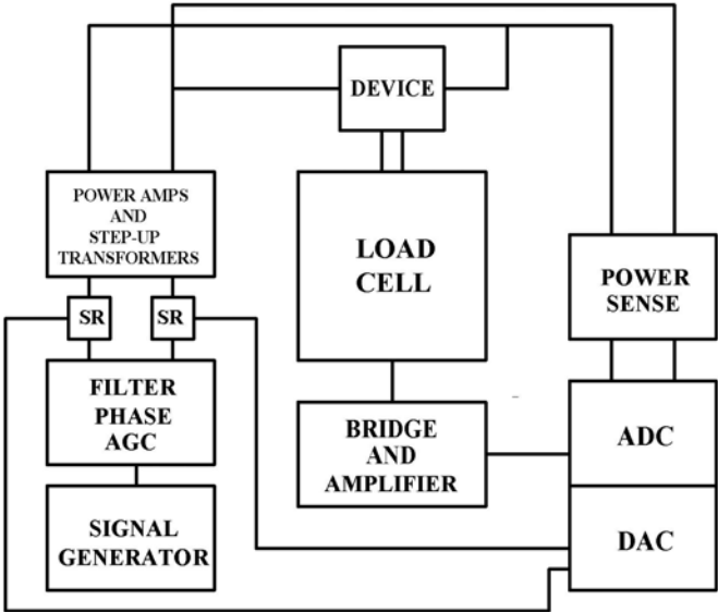
Figure 6: A schematic diagram of the chief electronic circuits in the apparatus.
