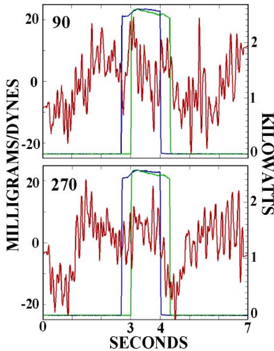
Figure 9: The 90 and 270 degrees results obtained when the polarity of the current in the inductors was reversed at the plug in the cage.
