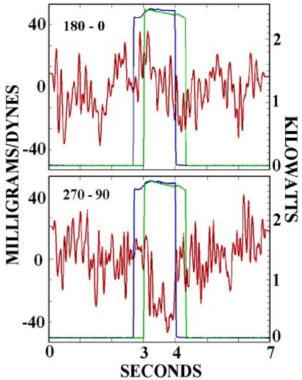
Figure 8: Differenced results for 180 minus 0 degrees and 270 minus 90 degrees. Note the prompt effect in the 270 minus 90 degrees data.
