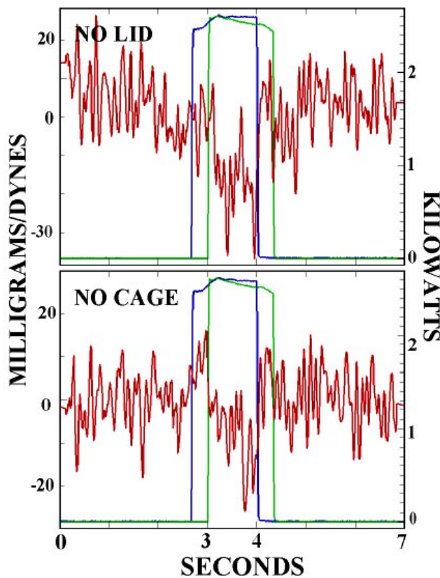
Figure 11: The 270 minus 90 degrees results obtained with all or part of the Faraday cage removed.
