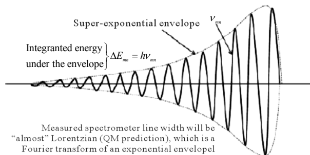
Figure 2. Photons are classical wave packets with a unique carrier frequency with a semi-exponentially decaying envelope. The model supports classical and QM observations.
