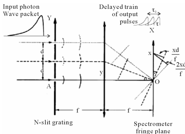
Figure 1. Pulse replication by grating and their temporally delayed superposition by a lens L in on a detector at the measurement plane.
