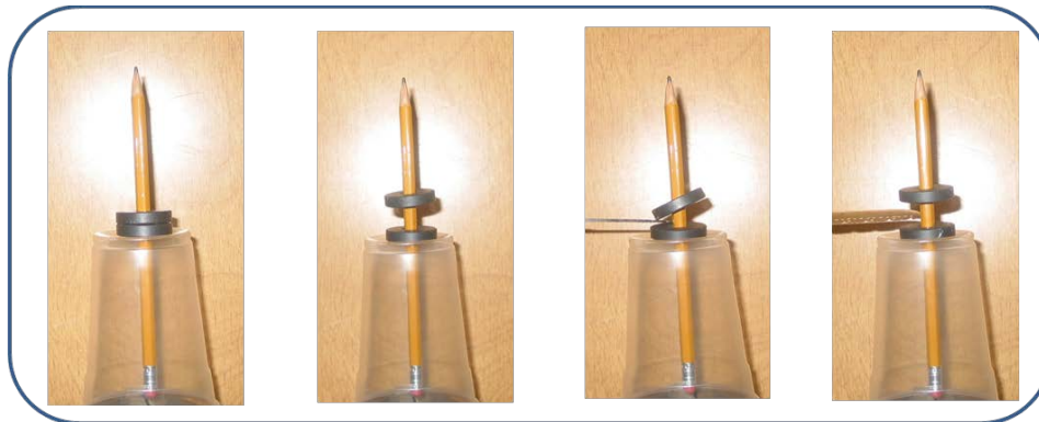
Annular magnets with same polarity repels each other. Space between them has “magnetic tension” that helps the upper magnet floating against gravitational tension.
